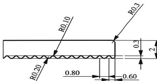
DETAIL C SCALE 5 : 1
